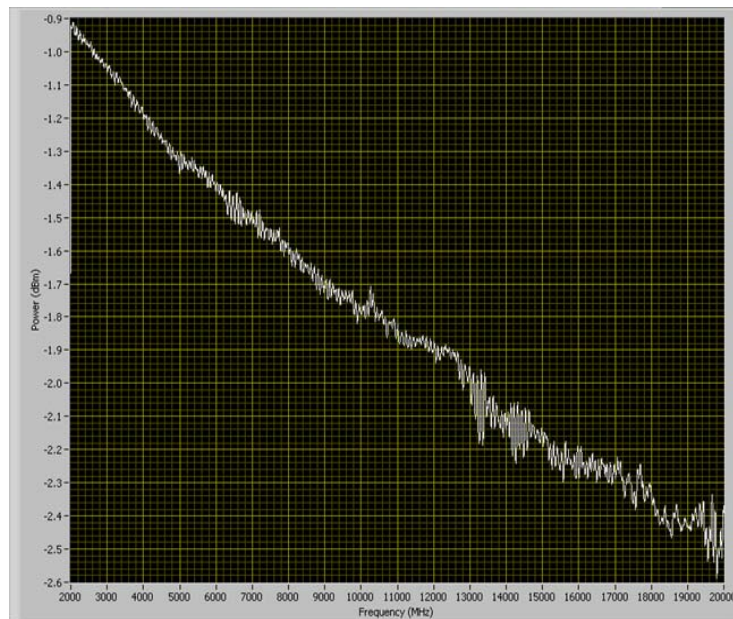
Figure 1: Cable losses without any correction applied
