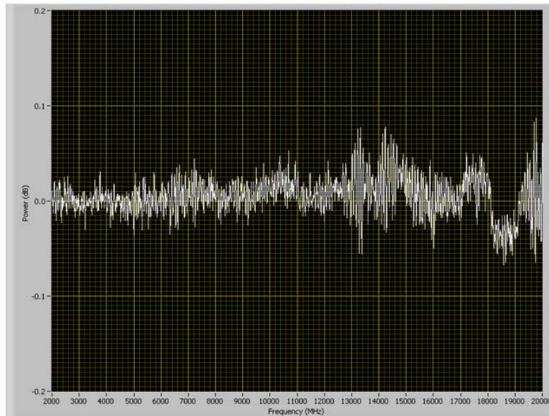
Figure 2: Error in corrected output power after the Cable Calibration correction has been applied
