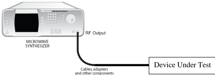
Figure 15: Cable Cal applied to correct for external path losses.
