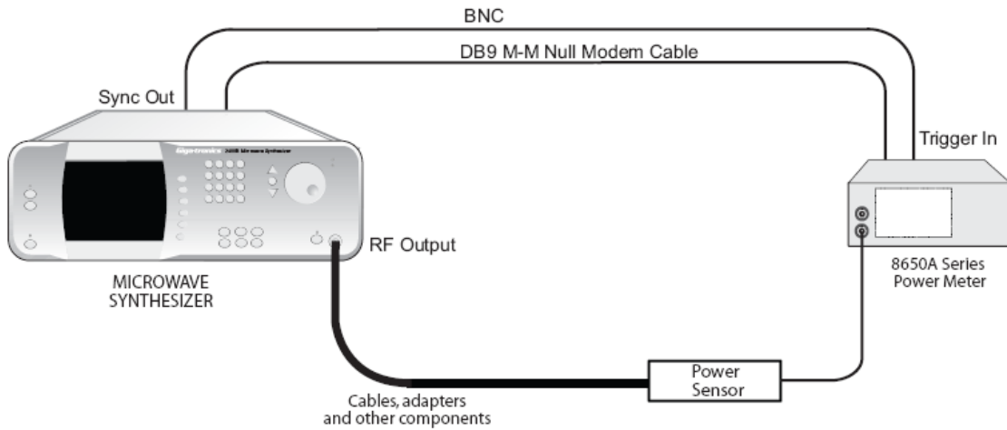
Figure 8: Cable Cal Equipment Setup
